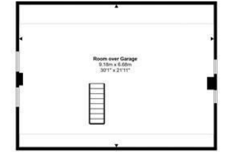
Garage First Floor Approx 81 sq m / 869 sq ft
